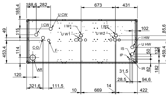
VER. RIP. FRONTALE E RETRO FRONT AIR AND BACK AIR SUCTION
